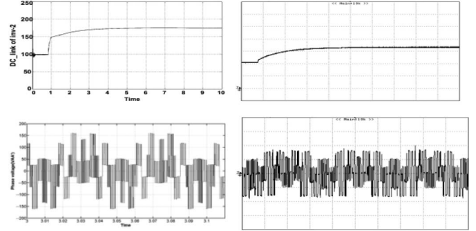
Fig. 2. (a) Direction of charging currents when both of the inverters are switched with the vector (+ — —). (b) Simulated and dc-link voltage of inverter-2 (left) and experimentally obtained dc-link voltage of inverter-2, scale: X-axis: 5 s/div; Y-axis: 50 V/div. (c) Simulated result of the actual motor phase voltage (left) experimentally obtained result of the actual motor phase voltage (right), scale: X-axis: 10 ms/div (for both); Y-axis: 50 V/div (left) 100 V/div (right).
