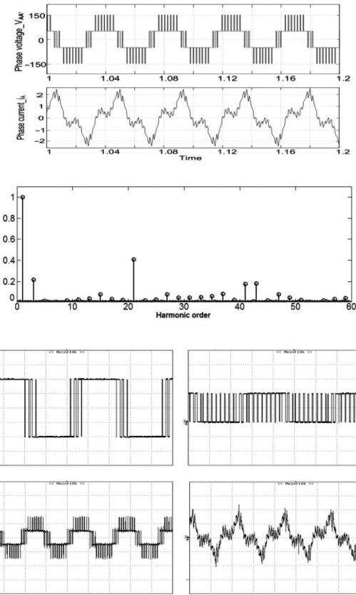
Fig. 7. (a) Simulated results of motor phase voltage and current. (b) Normalized harmonic spectrum of the difference in a-phase pole voltages for center spaced SVM at m_a = 0.4 . (c) Experimentally obtained result (right) of A-phase pole voltage of inverter-2 for an m_a = 0.4 , scale: X-axis: 10 ms/div; Y-axis: 50/div. (d) Experimental motor phase voltage (left) and motor phase current (right) for m_a = 0.4 with the center-spaced SVPWM technique (voltage scale: X-axis: 20 ms/div; Y-axis: 100 V/div and current scale: X-axis: 20 ms/div; Y-axis: 1 A/div).
