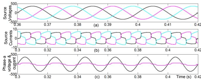
Fig. 3. Simulation results without DSTATCOM (a) source voltages, (b) source/load currents, (c) phase-a source voltage & current.
