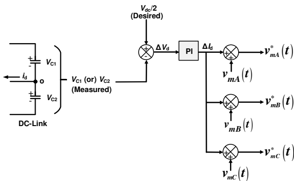
Fig. 7. DC-link capacitor voltage control.
