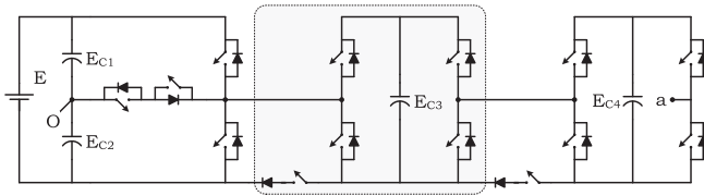
FIGURE 28. Hybrid seven-level SC with stacked configuration.
