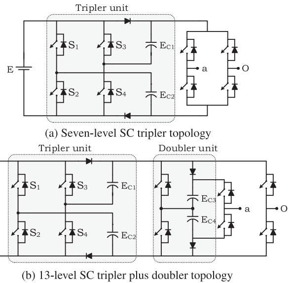
FIGURE 20. H-bridge based SC topologies.
