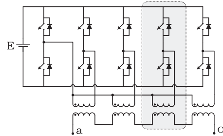
FIGURE 32. Single-source transformer based shared leg topology.
