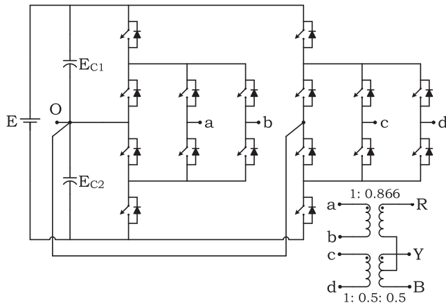
FIGURE 33. Transformer based two-phase topology.
