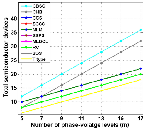
FIGURE 37. Comparison of TSV and total semiconductor count in generalized topologies.
