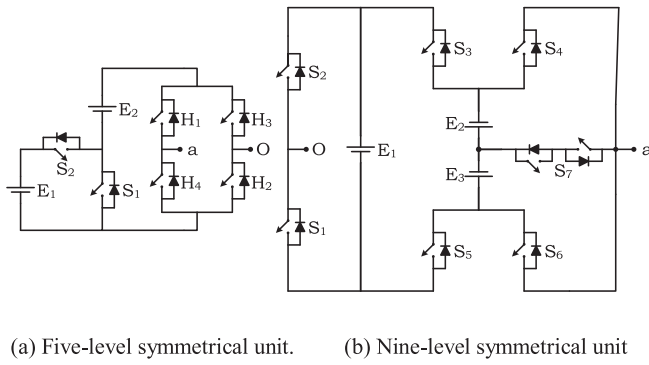
FIGURE 10. Symmetrical unit-based RSC-MLIs topologies.
