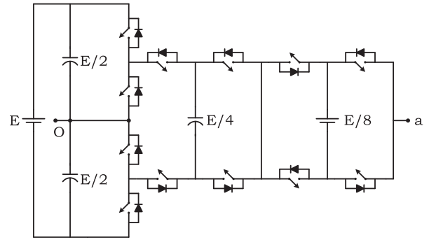
FIGURE 7. A hybrid 11-level configuration by stacking 5-level ANPC (primary) and FC module (secondary).
