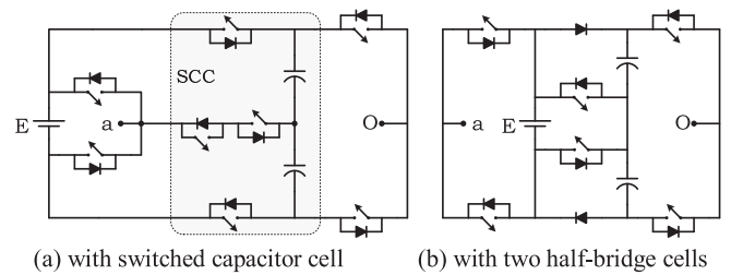
FIGURE 21. Five-level SC units.
