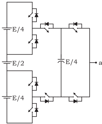
FIGURE 8. Five-level hybrid flying-capacitor (5L-HFC) inverter.
