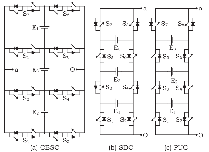
FIGURE 5. Topologies with ladder-based structures.
