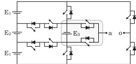
FIGURE 16. An extended H-bridge T-type topology [103].
