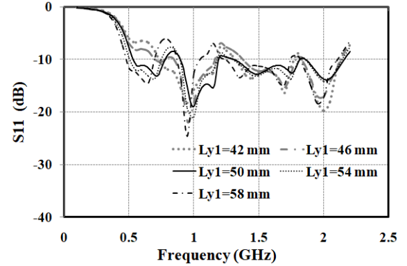
Fig. 5. Simulated S11 for variation in L_{y1} of the antenna.
