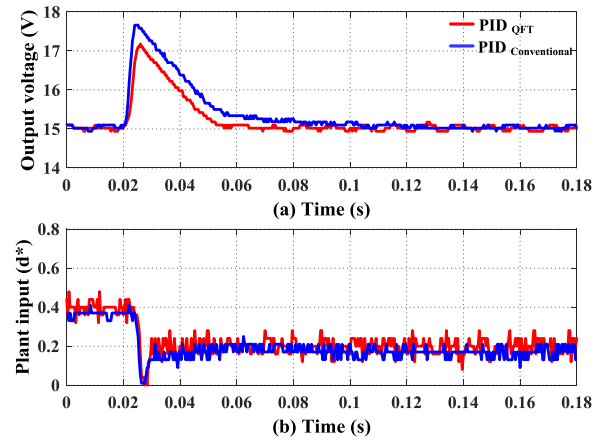
Fig. 8. Regulatory responses for input voltage variation from 10 V to 13 V at nominal load: (a) Output voltage (b) Plant input.
