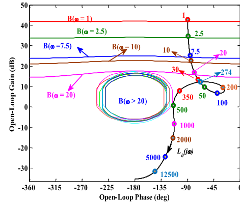
Fig. 3. Nominal loop shaping plot for the DC-DC boost converter.
