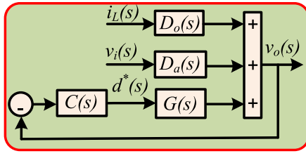
Fig. 2. Feedback control for disturbance rejection problem of Boost converter.
