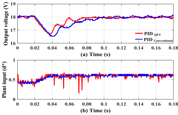
Fig. 10. Regulatory responses for a for input voltage variation from 10 V \rightarrow 7 V at a set-point of 18 V: (a) Output voltage (b) Plant input.
