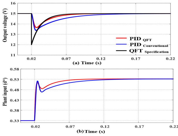
Fig. 4. Regulatory behaviour in linear simulations for a change in input source voltage from 10 V to 7 V: (a) Output voltage, and (b) Plant input ( d^* ).
