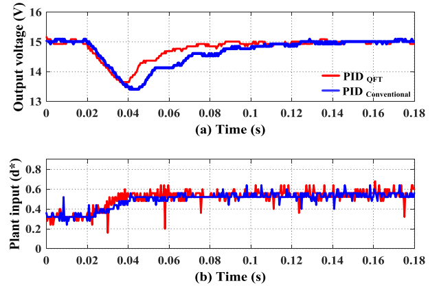
Fig. 7. Regulatory responses for input voltage variation from 10 V to 7 V at nominal load: (a) Output voltage (b) Plant input.
