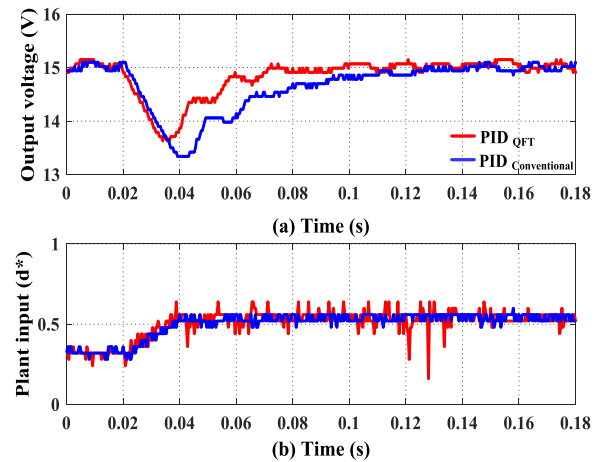
Fig. 9. Regulatory responses for input voltage variation from 10 V to 7 V at a load current of 0.2A: (a) Output voltage (b) Plant input.
