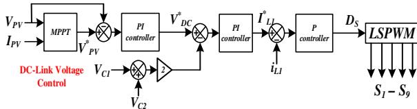
Fig. 4. Closed loop controller.
