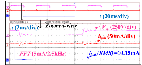
Fig. 14. Experimental results of parasitic capacitor voltage ( V_{cp} ), leakage current ( i_{leak} ) of the PV source, and harmonic spectrum of leakage current.
