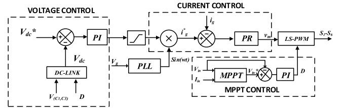
Fig. 6. Control scheme for grid-tied 5L-qZSI.
