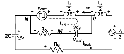
Fig. 8. Equivalent circuit of common-mode model.
