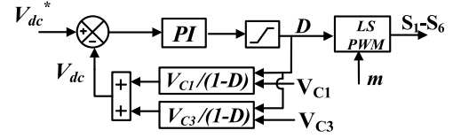
Fig. 5. Indirect dc-link voltage regulation of the proposed 5L-qZSI.
