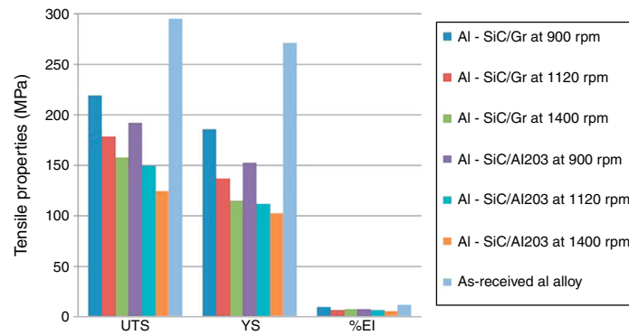
Fig. 9 – Comparison of tensile properties of aluminum alloy surface composites.
