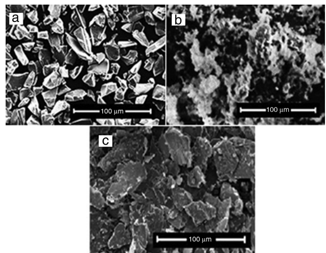
Fig. 1 – SEM micrographs of as-received: (a) SiC, (b) \text{Al}_2\text{O}_3 and (c) Gr particles.
