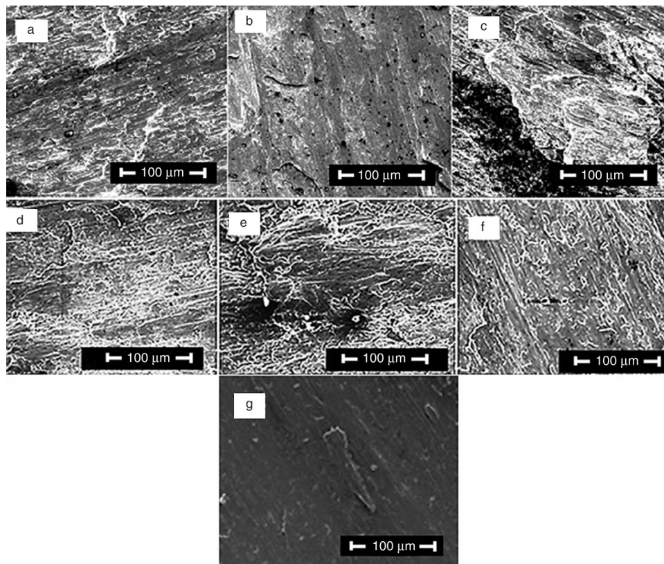
Fig. 8 – Worn morphology of the surface hybrid composites: (a) Al-SiC/Gr at 900 rpm, (b) Al-SiC/Gr at 1120 rpm, (c) Al-SiC/Gr at 1400 rpm, (d) Al-SiC/ \text{Al}_2\text{O}_3 at 900 rpm, (e) Al-SiC/ \text{Al}_2\text{O}_3 at 1120 rpm, (f) Al-SiC/ \text{Al}_2\text{O}_3 at 1400 rpm and (g) as-received aluminum alloy.
