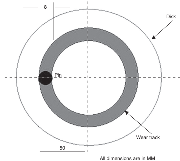
Fig. 4 – Schematic configuration of pin-on-disk tribo-meter.
