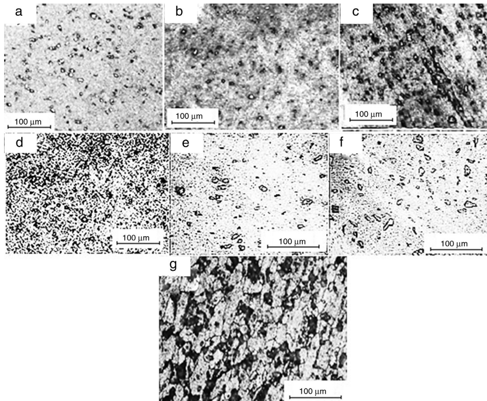
Fig. 5 – Optical microstructures of the surface hybrid composites: (a) Al-SiC/Gr at 900 rpm, (b) Al-SiC/Gr at 1120 rpm, (c) Al-SiC/Gr at 1400 rpm, (d) Al-SiC/Al 2 O 3 at 900 rpm, (e) Al-SiC/Al 2 O 3 at 1120 rpm, (f) Al-SiC/Al 2 O 3 at 1400 rpm and (g) as-received aluminum alloy.
