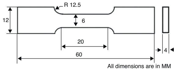
Fig. 3 – Schematic of tensile specimen.
