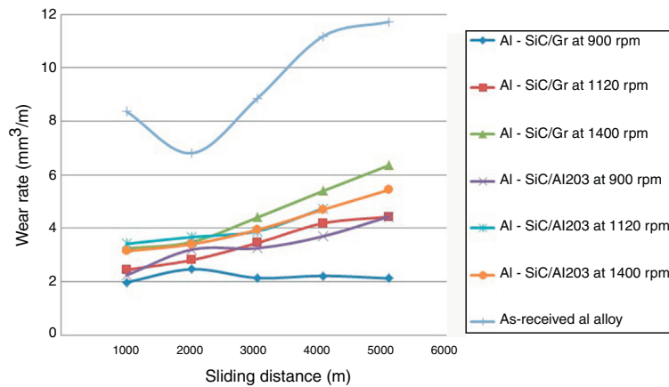
Fig. 7 – Variation of wear rate with respect to the sliding of aluminum alloy surface composites.
