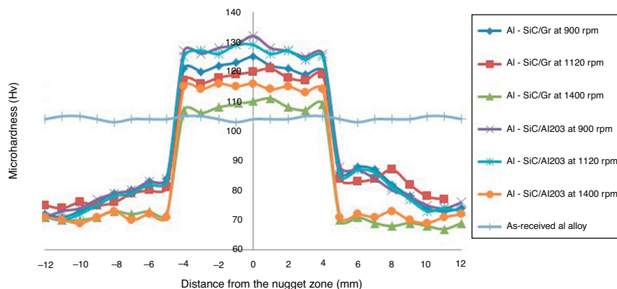
Fig. 6 – Microhardness survey of aluminum alloy surface hybrid composites.
