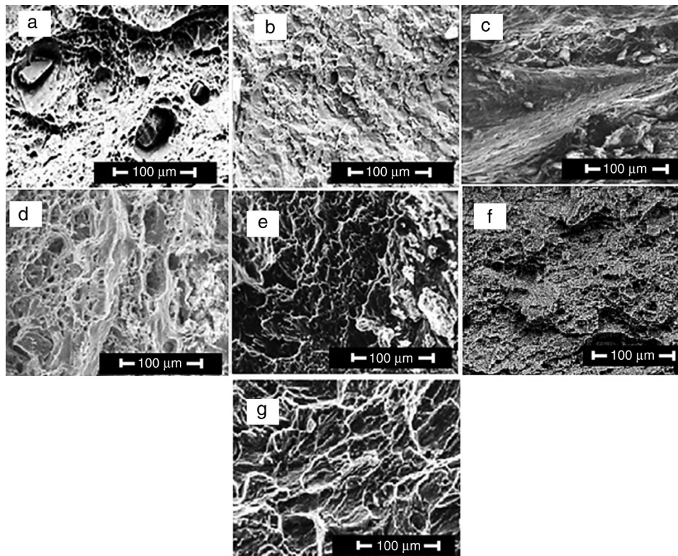
Fig. 10 – Fracture features of (a) Al-SiC/Gr at 900 rpm, (b) Al-SiC/Gr at 1120 rpm, (c) Al-SiC/Gr at 1400 rpm, (d) Al-SiC/Al 2 O 3 at 900 rpm, (e) Al-SiC/Al 2 O 3 at 1120 rpm, (f) Al-SiC/Al 2 O 3 at 1400 rpm and (g) as-received aluminum alloy.
