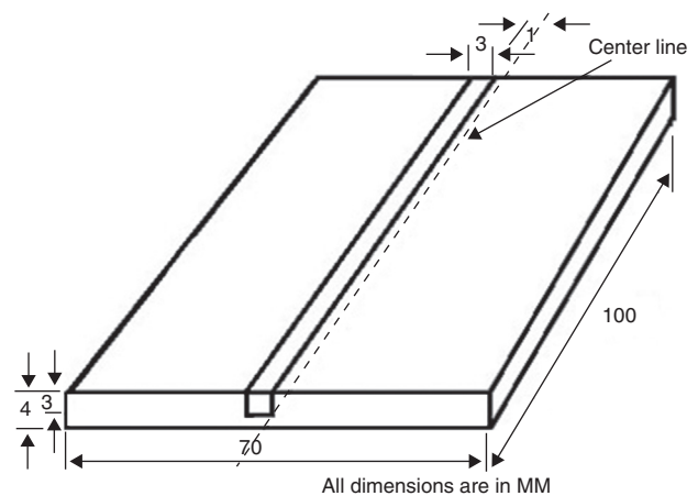
Fig. 2 – Schematic of aluminum alloy plate for FSP.
