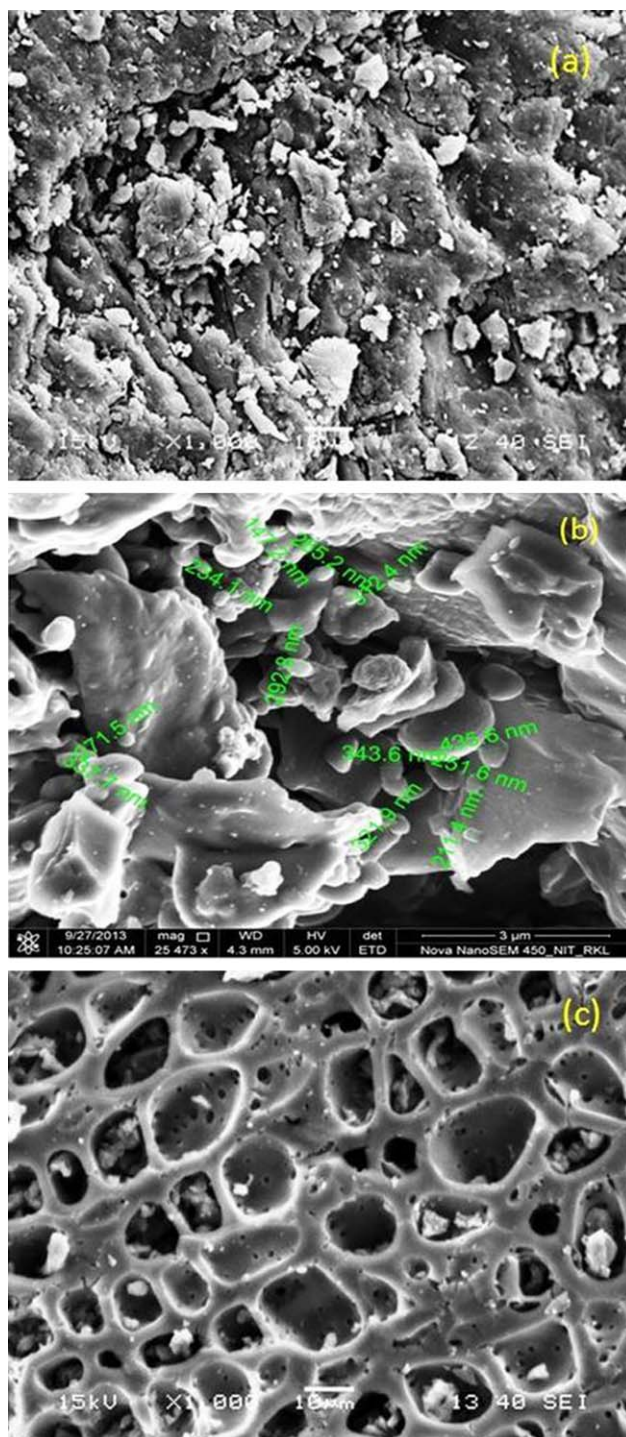
Figure 11. (a) Raw wood apple shell particles. (b) Carbon black wood apple shell particles (600°C). (c) Carbon black wood apple shell particles (800°C). [Color figure can be viewed in the online issue, which is available at wileyonlinelibrary.com .]
