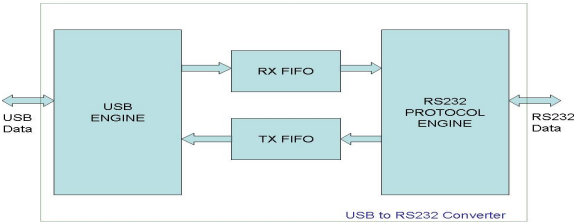
Fig 1.RS232 to USB Interface Diagram
