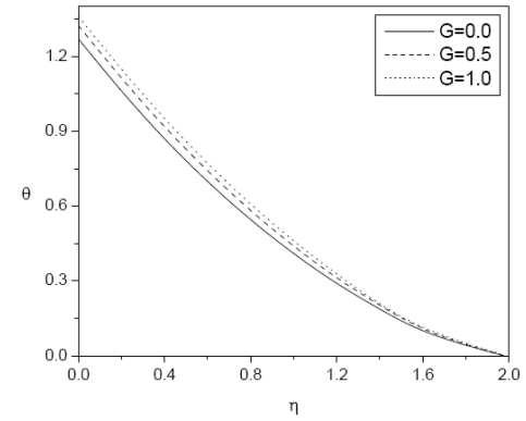
Figure 12. Temperature profiles for various values of G with N = 0.5 , Le = 0.5 , n = 0.5 , M = 1 , \varepsilon_1 = 0.2 , \varepsilon_2 = 0.8 .
