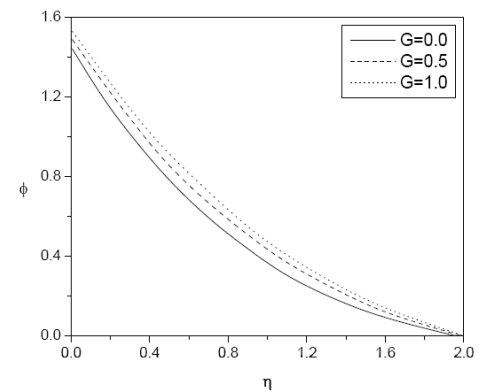
Figure 13. Concentration profiles for various values of G with N = 0.5 , Le = 0.5 , n = 0.5 , M = 1 , \varepsilon_1 = 0.2 , \varepsilon_2 = 0.8 .
