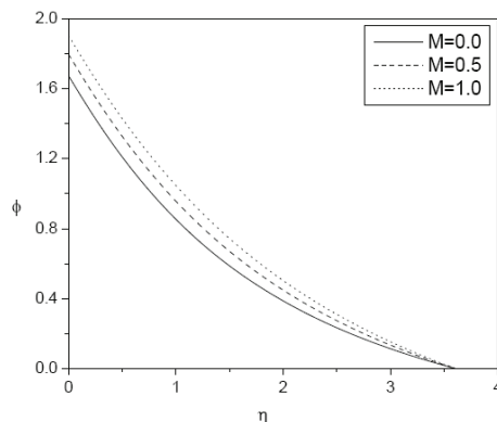
Figure 10. Concentration profiles for various values of M with N = 0.5 , Le = 0.5 , n = 0.5 , G = 1 , \varepsilon_1 = 0.2 , \varepsilon_2 = 0.8 .
