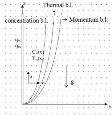
Figure 1. Physical model and coordinate system.
