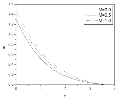
Figure 9. Temperature profiles for various values of M with N = 0.5 , Le = 0.5 , n = 0.5 , G = 1 , \varepsilon_1 = 0.2 , \varepsilon_2 = 0.8 .
