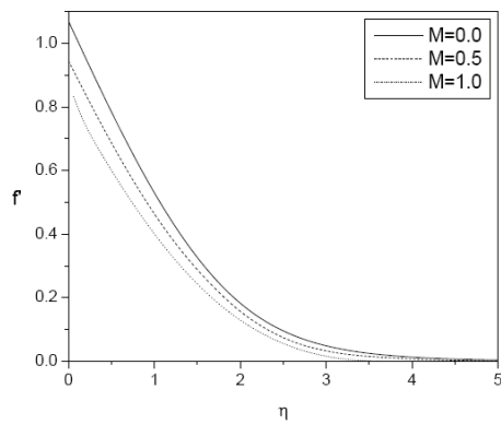
Figure 8. Velocity profiles for various values of M with N = 0.5 , Le = 0.5 , n = 0.5 , G = 1 , \varepsilon_1 = 0.2 , \varepsilon_2 = 0.8 .
