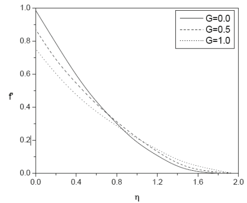
Figure 11. Velocity profiles for various values of G with N = 0.5 , Le = 0.5 , n = 0.5 , M = 1 , \varepsilon_1 = 0.2 , \varepsilon_2 = 0.8 .
