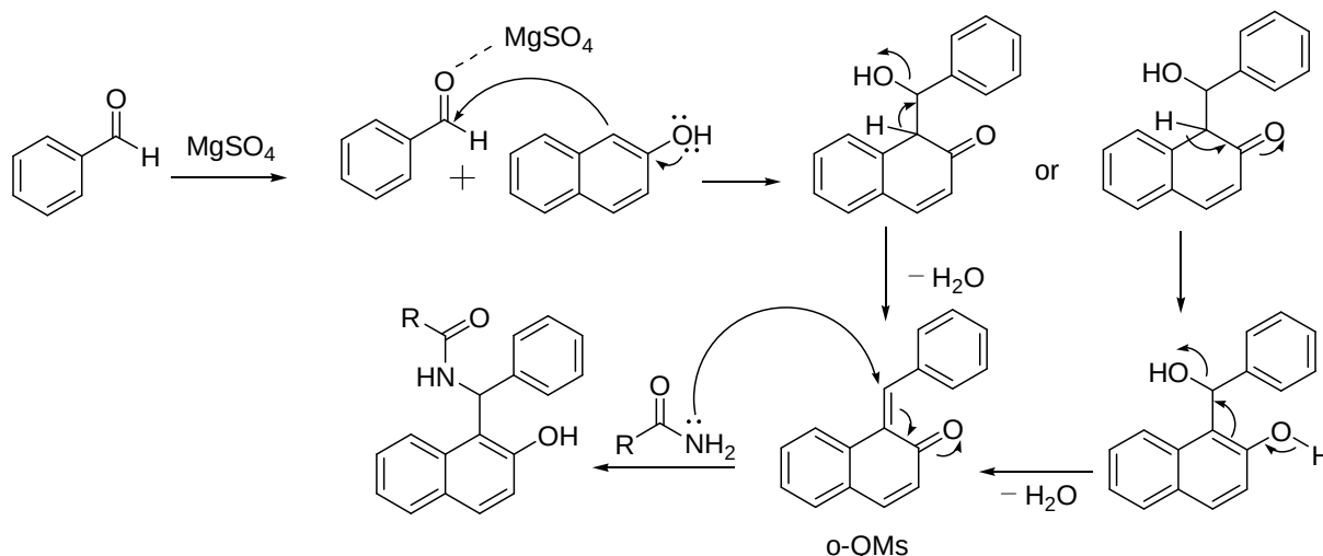
Figure 2. Possible mechanism for the synthesis of amidoalkyl naphthols by \text{MgSO}_4
