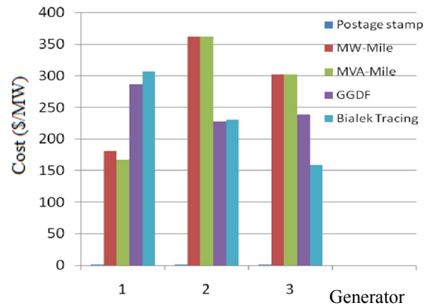
Fig. 4. Comparison of 6 bus system results for different methods
