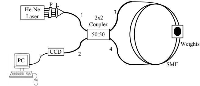
Fig.1 Experimental set up of the Fiber optic Sagnac Interferometer.
