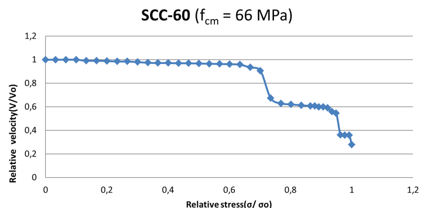
Fig. 6. Change in UPV with increase in stress level in self-compacting concrete class \approx C55/67
