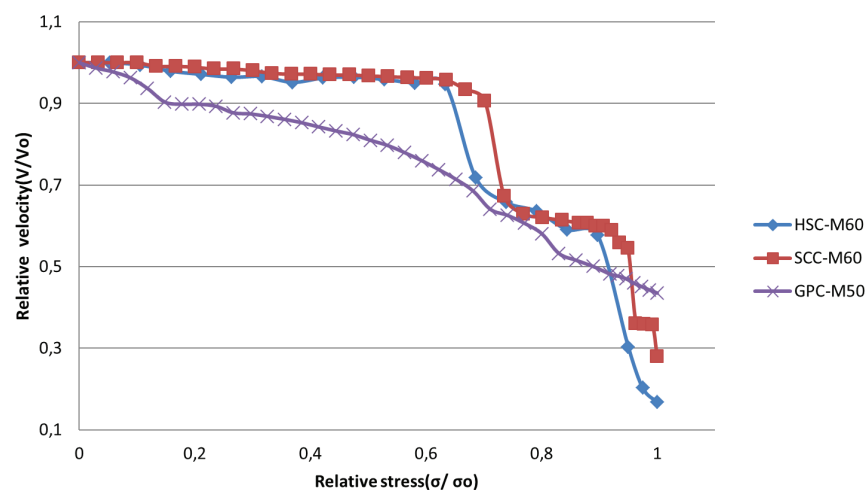
Fig. 9. Comparison of change in UPV with increase in stress level in different concretes of high class.
