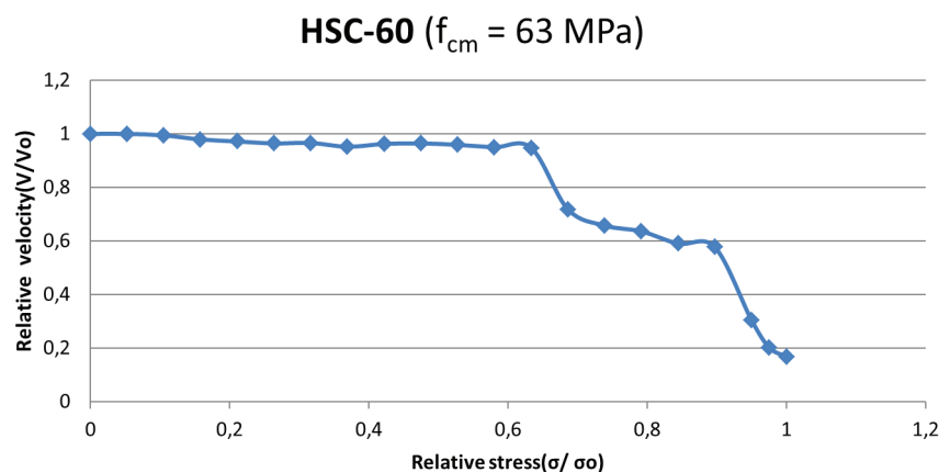
Fig. 5. Change of UPV with increase of stress level in high-strength concrete class \approx C55/67
