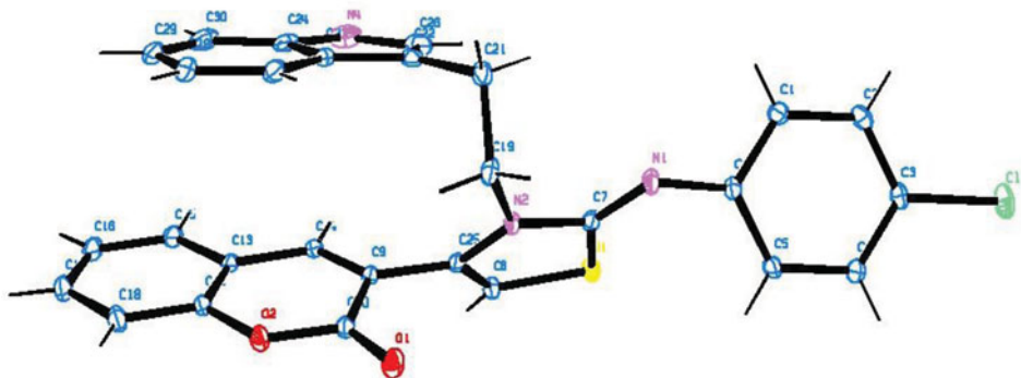
Figure 1 ORTEP Representation of Compound 4b .
