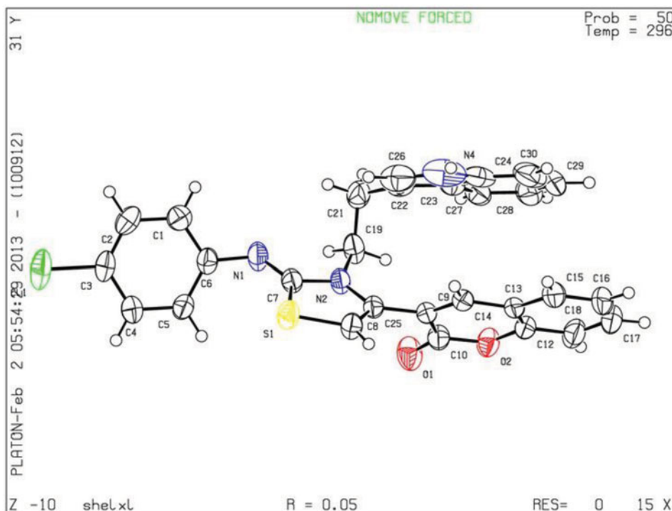
Figure 2 PLATON Representation of Compound 4b . Thermal Ellipsoids are drawn at 50% probability level.
