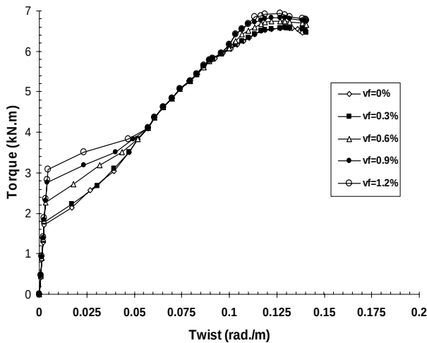
Figure 6. Torque twist response of completely over reinforced members
