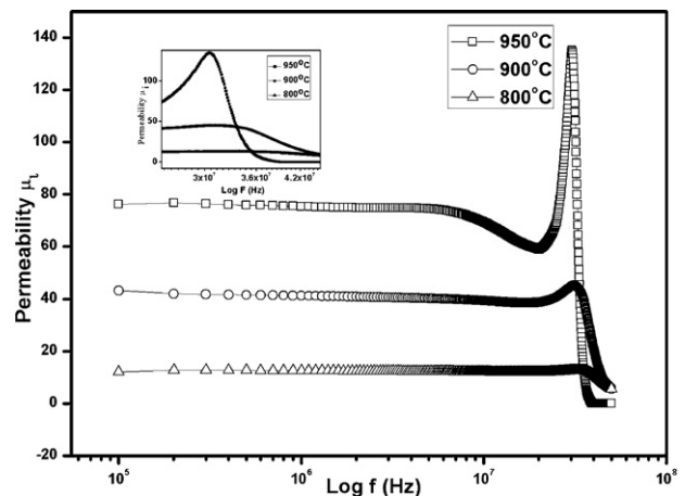
Fig. 7. Frequency dispersion of permeability for the sintered samples 800 °C (a), 900 °C (b) and 950 °C. The inset shows high frequency dispersion of permeability.
