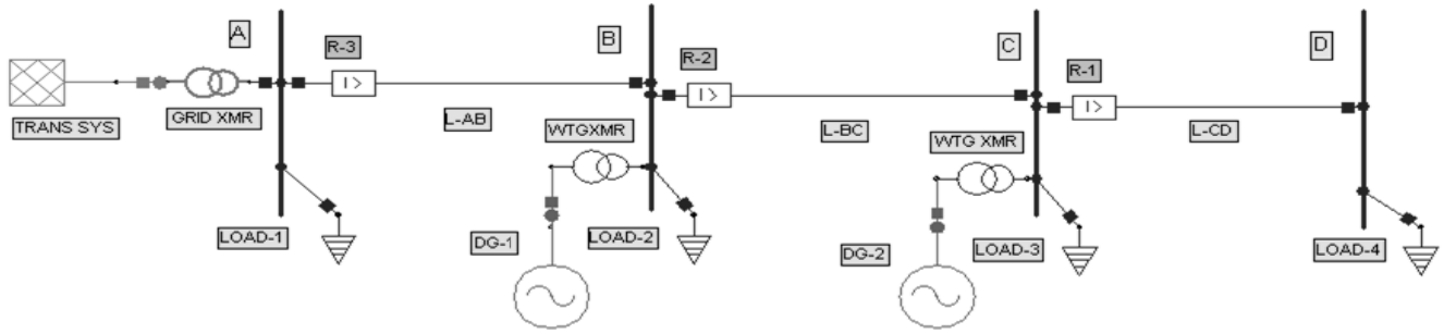
Figure 5. Two DG Connected to Radial System
