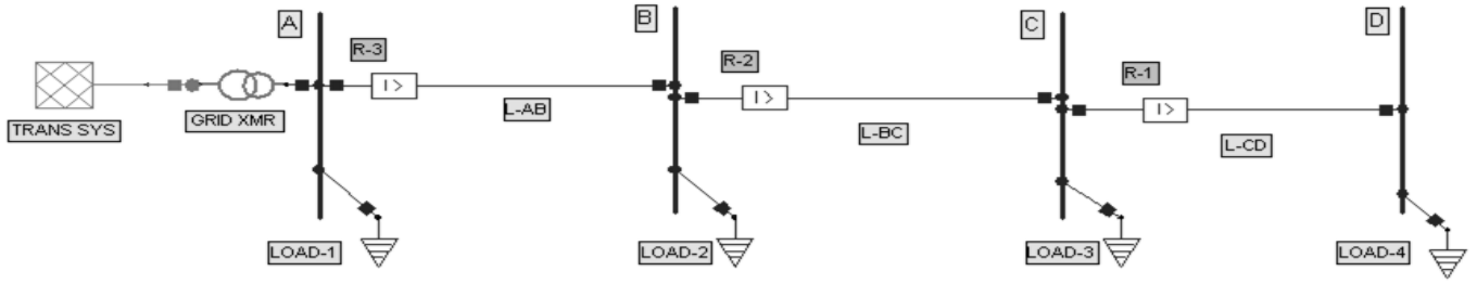
Figure 2. Distribution system with out distribution generation
