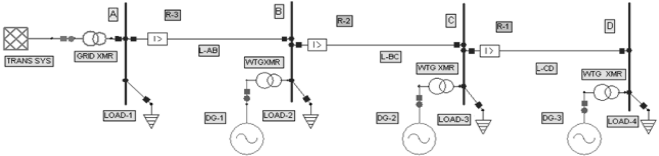
Figure 6. Three DG Connected to Radial System
