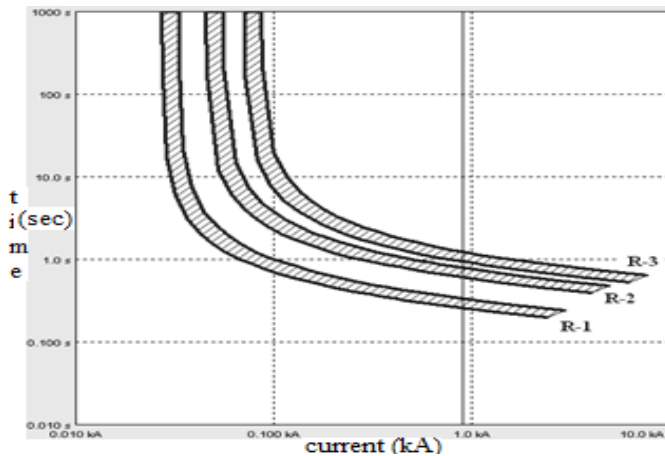
Figure 1. Selectivity diagram of Relays when fault applied to bus-D (with-out DG case)
