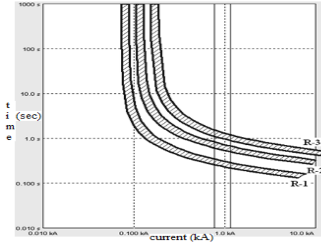
Figure 4. Selectivity Diagram of Relays when fault applied to Bus-D (with single DG case)
