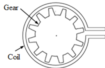
Fig. 1(a). Gear and coil arrangement
