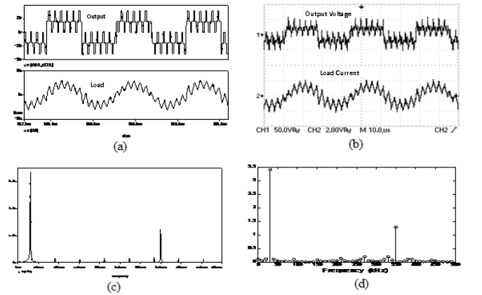
Fig. 5. Simulation and experimental results of v_0, i_0 and FFTs of output current (a) Simulation waveforms of v_0 and i_0 (b) Experimental waveforms of v_0 and i_0 (c) FFT of simulated waveform of i_0 (d) FFT of experimental waveform of i_0
