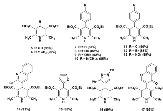
Figure-1. Different dihydropyridine (DHP) derivatives ( 5-17 )
