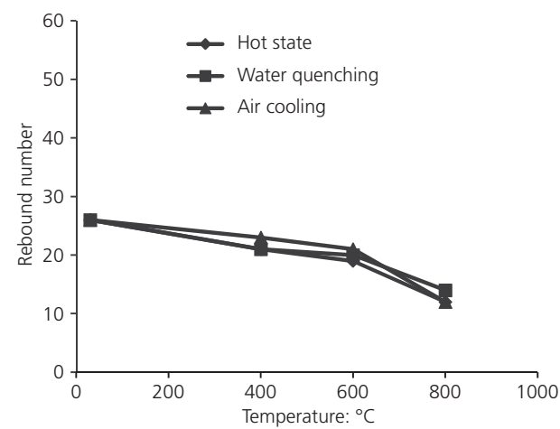
Figure 5. Rebound number plotted against temperature for M20 grade NC
