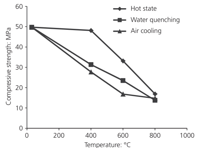
Figure 3. Compressive strength temperature for M40 grade NC
