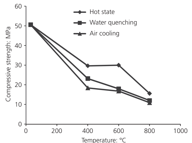
Figure 4. Compressive strength plotted against temperature for M40 grade SCC
