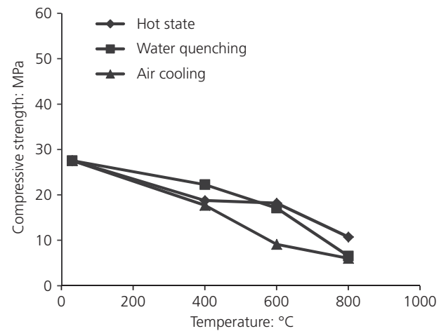
Figure 2. Compressive strength plotted against temperature for M20 grade SCC
