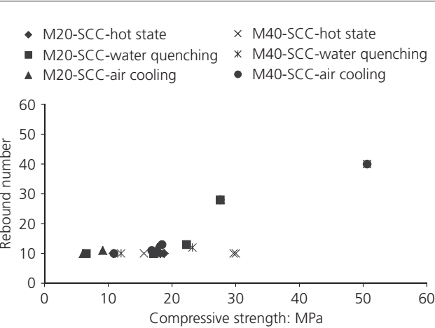
Figure 10. Rebound number plotted against compressive strength for SCC
