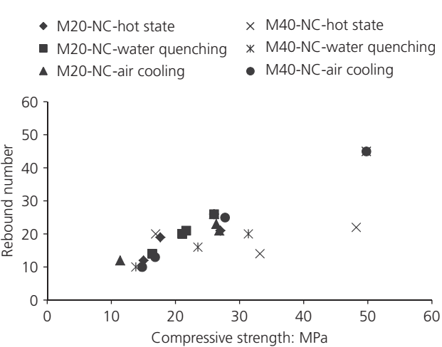
Figure 9. Rebound number plotted against compressive strength for NC
