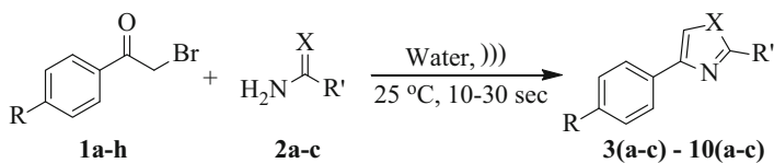
Scheme 1 Synthesis of 2,4-disubstituted-1,3-thiazoles and selenazoles with phenacyl bromides (1a–h)
