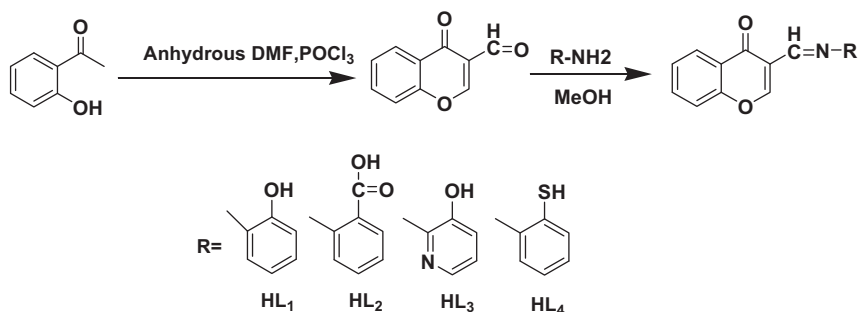
Scheme 1. Synthesis of Schiff base ligands.
