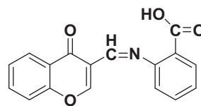
2-((4-oxo-4H-chromen-3-yl)methyleneamino)benzoic acid (HL 2 )
