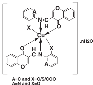
Fig. 5. Structure of Cu(II) complexes.
