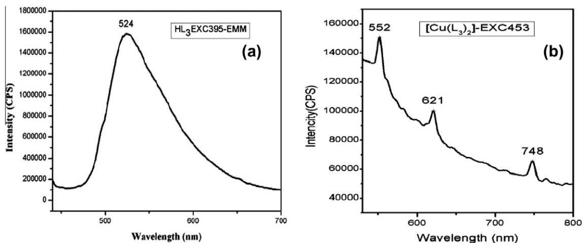
Fig. 6. Emission spectra of (a) HL 3 and (b) [Cu(L 3 ) 2 ].
