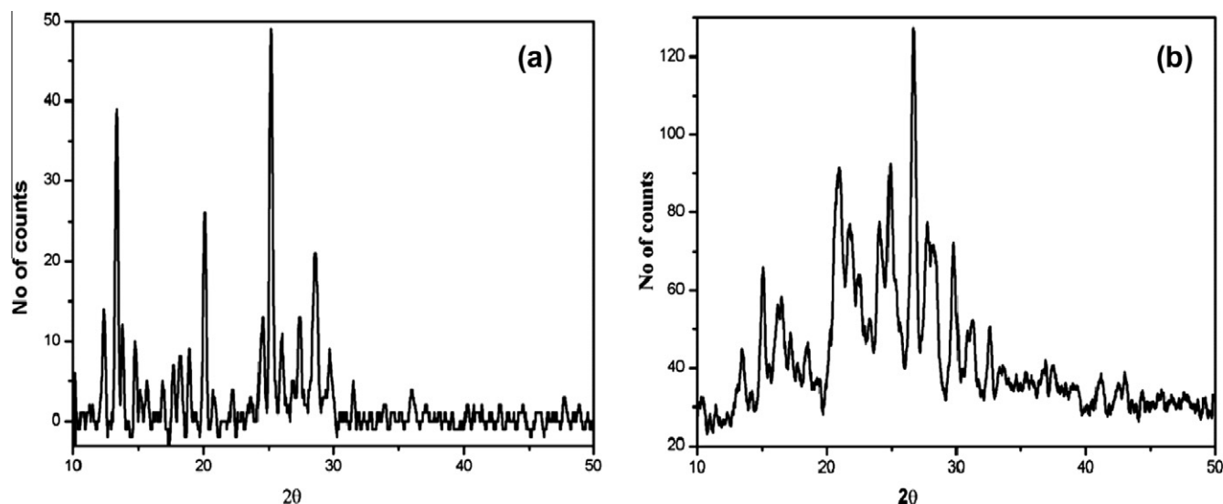
Fig. 7. PXRD patterns of (a) HL 3 and (b) [Cu(L 3 ) 2 ].
