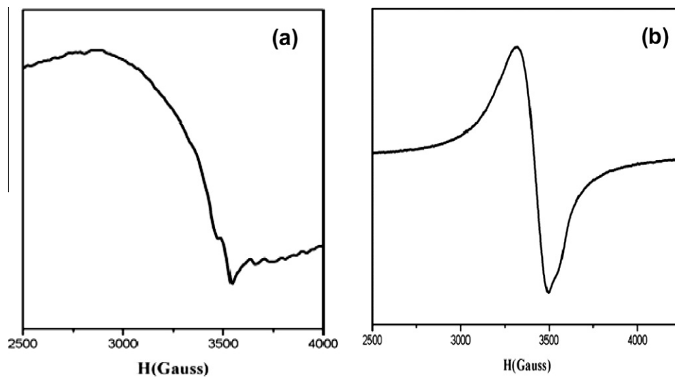
Fig. 3. ESR spectra of (a) [\text{Cu}(\text{L}_1)_2] \cdot 2\text{H}_2\text{O} and (b) [\text{Cu}(\text{L}_4)_2] .
