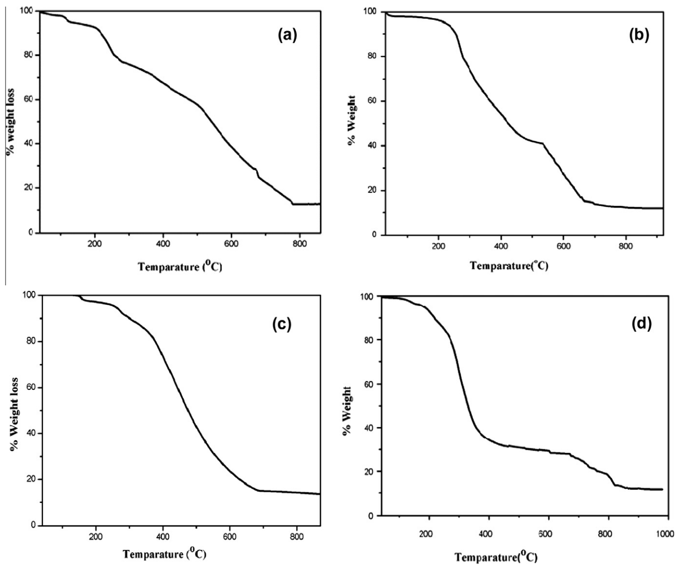
Fig. 4. TG graphs of (a) [\text{Cu}(\text{L}_1)_2] \cdot 2\text{H}_2\text{O} , (b) [\text{Cu}(\text{L}_2)_2] \cdot \text{H}_2\text{O} , (c) [\text{Cu}(\text{L}_3)_2] , and (d) [\text{Cu}(\text{L}_4)_2] .
