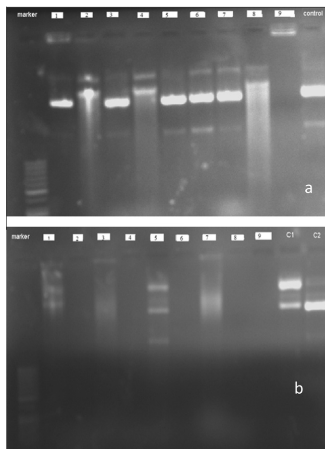
Fig. 9. DNA cleavage studies of ligands and their Cu(II) complexes. (a) DNA cleavage activity in the absence of H 2 O 2 . Lane 1: DNA + HL 1 , Lane 2: DNA + [Cu(L 1 ) 2 ].2H 2 O, Lane 3: DNA + HL 2 , Lane 4: DNA + [Cu(L 2 ) 2 ].H 2 O, Lane 5: DNA + HL 3 , Lane 6: DNA + [Cu(L 3 ) 2 ], Lane 7: DNA + HL 4 , Lane 8: DNA + [Cu(L 4 ) 2 ], Lane 9: DNA + FeSO 4 , Lane control: DNA alone. (b) DNA cleavage in the presence of H 2 O 2 . Lane 1: DNA + HL 1 + H 2 O 2 , Lane 2: DNA + [Cu(L 1 ) 2 ].2H 2 O + H 2 O 2 , Lane 3: DNA + HL 2 + H 2 O 2 , Lane 4: DNA + [Cu(L 2 ) 2 ].H 2 O + H 2 O 2 , Lane 5: DNA + HL 3 + H 2 O 2 , Lane 6: DNA + [Cu(L 3 ) 2 ] + H 2 O 2 , Lane 7: DNA + HL 4 + H 2 O 2 , Lane 8: DNA + [Cu(L 4 ) 2 ] + H 2 O 2 , Lane 9: DNA + FeSO 4 + H 2 O 2 , Lane C1: DNA + H 2 O 2 , Lane C2: DNA alone.
