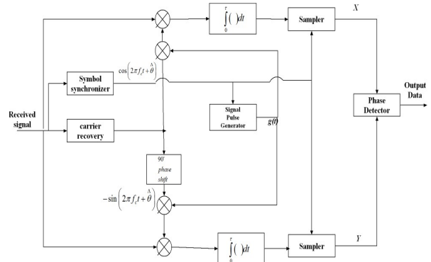
Fig. 1: Receiver Model
