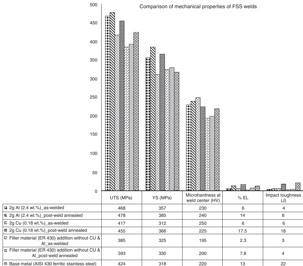
Fig. 4 – Graphical representation of mechanical properties of FSS welds.
