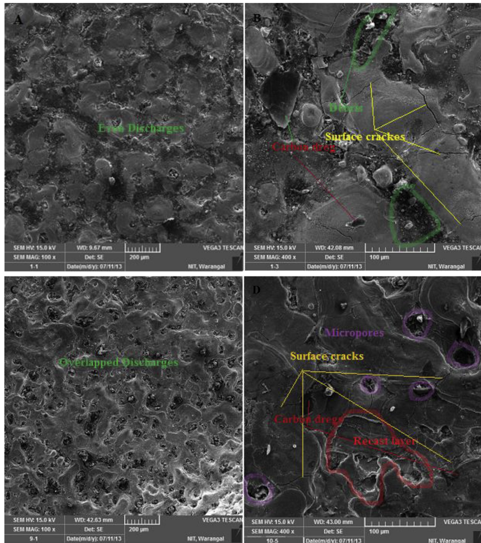
Fig. 8. A&B machined surface characteristics under discharge current of 10 A, Surfactant concentration 4 g/lit and graphite 4.5 g/lit. (At low surface roughness condition, (A) low magnification and (B) high magnification). C&D machined surface characteristics under discharge current of 20 A, Surfactant Concentration 6 g/lit and graphite 13.5 g/lit. (At high material removal rate condition, (C) low magnification and (D) high magnification).
