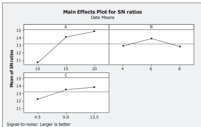
Fig. 4. S/N response graph for material removal rate.
