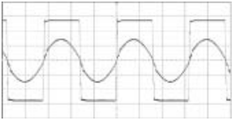
Fig. 12(a): BPS inverter output voltage and tank current (Voltage: 100 V/div., Current: 2 A/div., Time: 5 \mu secs./div.)
