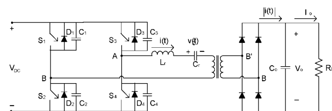
Fig. 5: Phase-modulated series resonant converter
