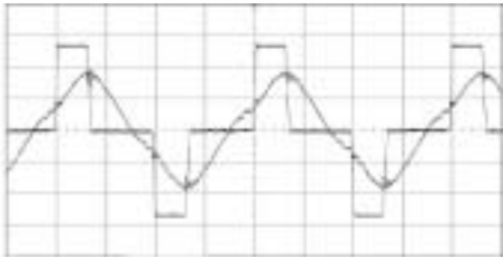
Fig. 13(a): FPS inverter output voltage and tank current (Voltage: 100 V/div., Current: 0.5 A/div., Time: 1 \mu sec./div.)
