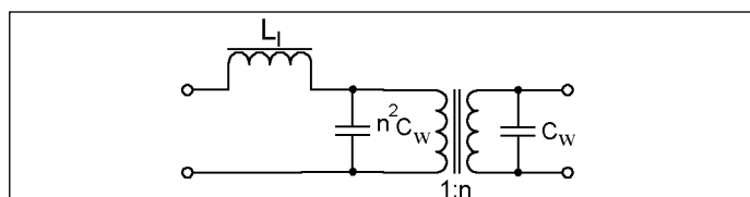
Fig. 2: HV transformer equivalent ckt
