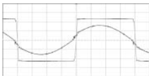
Fig. 17: Waveform showing effect of winding capacitance (Voltage: 200 V/div., Current: 1 A/div., Time: 2 msecs./div.)
