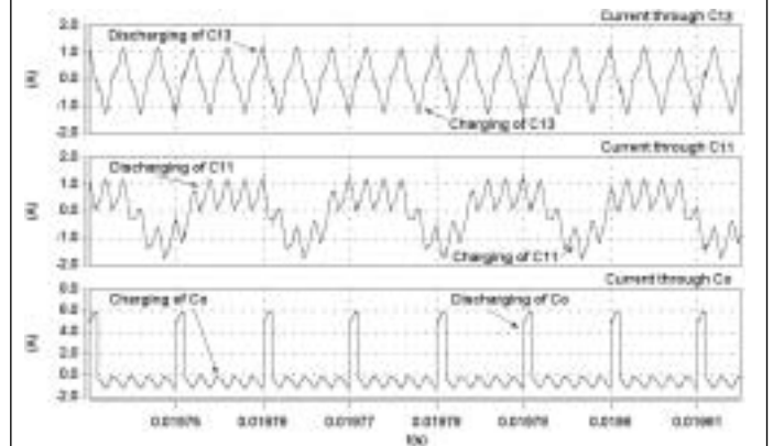
Fig. 11(b): Output waveforms for C_B:C_F = 15:1 , PRF = 100 kHz
