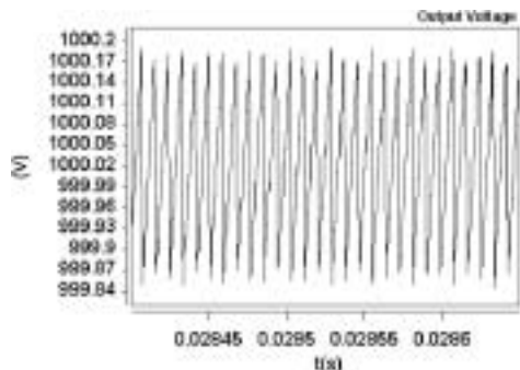
(b) PRF = 115 kHz
