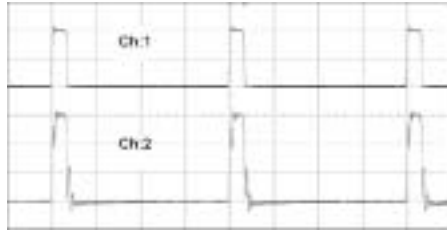
Fig. 15 (c): Experimental load waveforms (Ch:1:Voltage, Ch:2: Current)(Voltage: 500 V/div., Current: 2 A/div., Time: 2 μsecs./div.)
