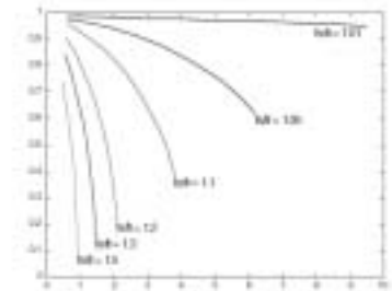
(c) Voltage gain vs. load current (varying f_s/f_r )
