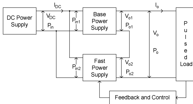
Fig. 10(a): Block diagram of OVM converter
