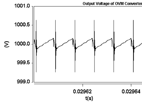
Fig.15(b): Parasitic effect on output voltage
