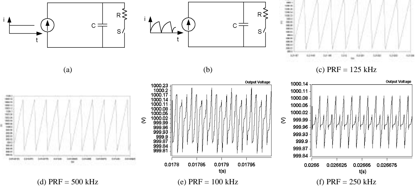
Fig. 9: Beat frequency oscillations
