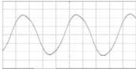
Fig. 13(b): FPS resonant capacitor voltage (Voltage: 100 V/div., Time: 1 \mu sec./div.)
