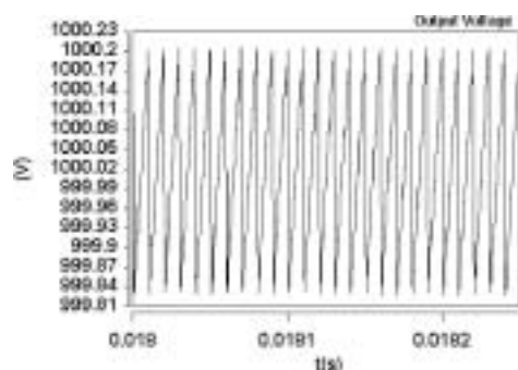
(a) PRF = 100 kHz
