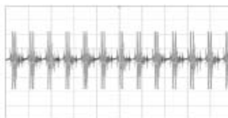
(f) Voltage: 1 V/div., Time: 5 \mu secs./div., PRF = 250 kHz
