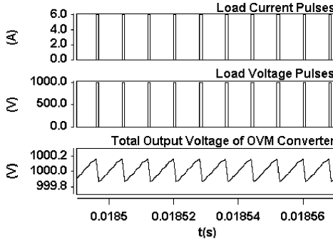
Fig. 15(a): Simulated load waveforms
