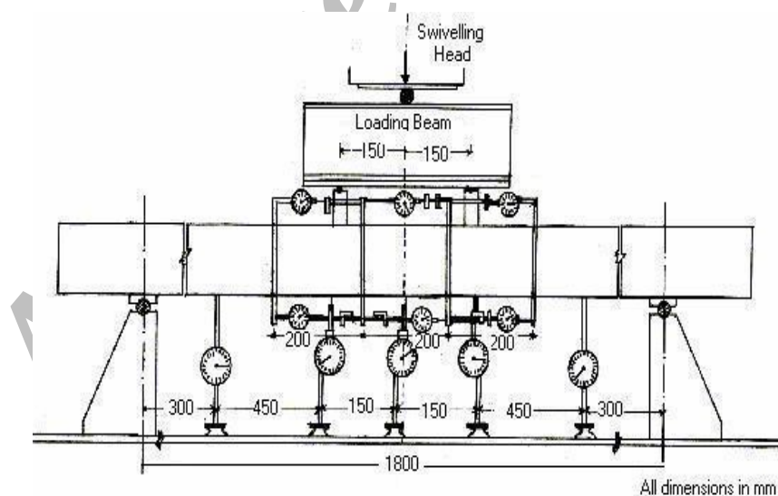
Figure 1. Test Setup
