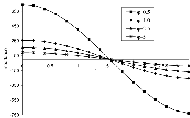
Fig. 3. Effect of \varphi on impedance with k = 0.1 , \gamma = 0.5 , \alpha = 1.5 , \sigma = 0.5 , \varepsilon = 0.15 .
