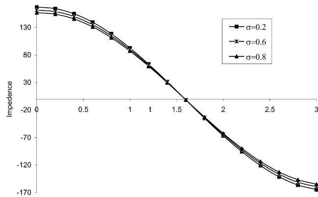
Fig. 4. Effect of \sigma on impedance with k = 0.1 , \varphi = 2.5 , \gamma = 0.5 , \alpha = 1.5 , \varepsilon = 0.15 .
