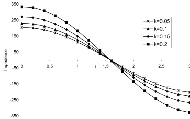
Fig. 2. Effect of k on impedance with \varphi = 1.5 , \gamma = 0.5 , \alpha = 1.5 ; \sigma = 0.5 , \varepsilon = 0.1 .
