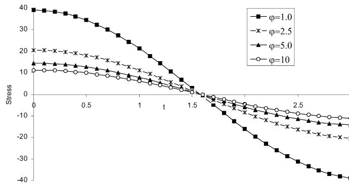
Fig. 6. Effect of \varphi on stress with k = 0.1 , \alpha = 2 , \sigma = 0.5 , \varepsilon = 0.1 .
