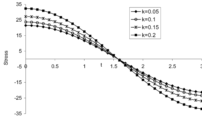
Fig. 5. Effect of k on stress with \varphi = 2 , \alpha = 2 , \sigma = 0.5 , \varepsilon = 0.1 .
