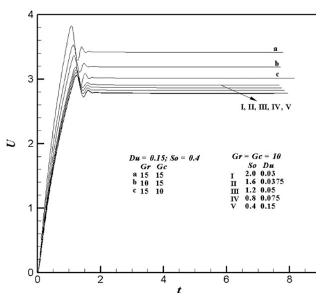
Fig. 7. The transient velocity for different dimensionless parameters with respect to time at (1.0, 1.6).
