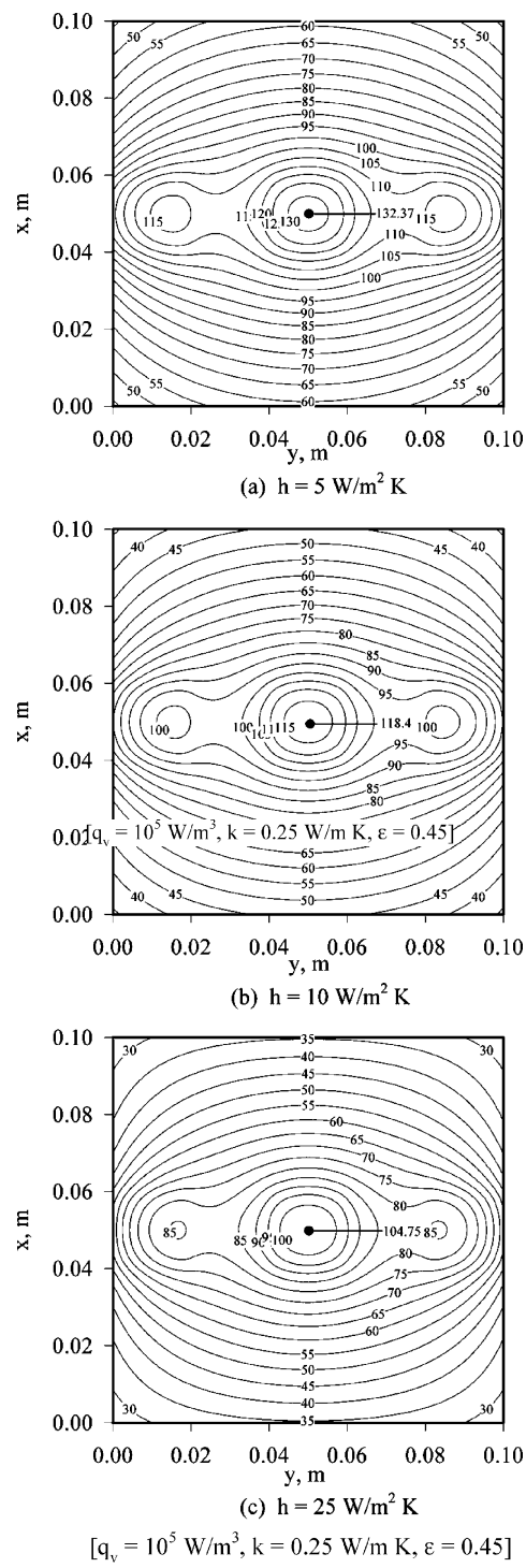
Figure 2. Isotherm plots for different values of convection heat transfer coefficient.
