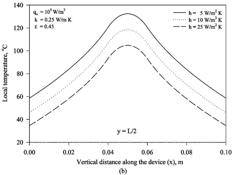
Figure 5. Local temperature profiles in the electronic device for different values of convection heat transfer coefficient.
