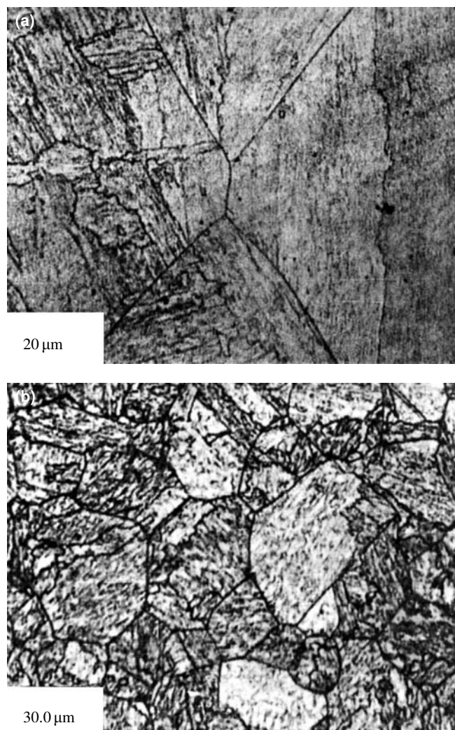
Fig. 4. Optical micrographs of T18Ni1700: (a) Solution annealed at 1200 °C and water quenched, and (b) material at (a) thermally cycled once between 875 °C and room temperature [29].
