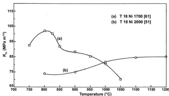
Fig. 6. Variation of fracture toughness with SA temperature.
