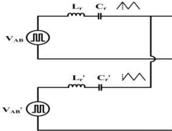
Fig. 2. Equivalent circuit of Proposed Converter
